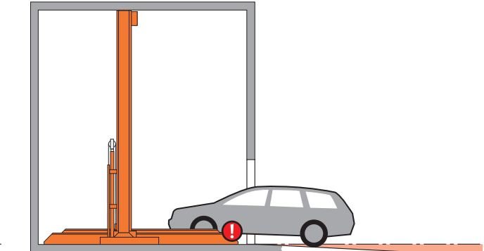
maximum ascending slope 14 %
