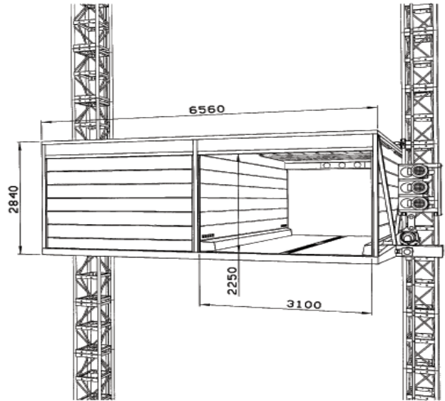
ARK PARKING LIFT TWO MAST VERSION POSITIONING
