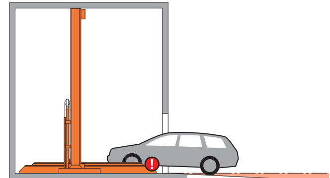
maximum ascending slope 14 %
