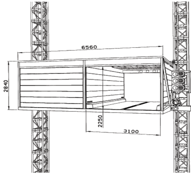
ARK PARKING LIFT TWO MAST VERSION POSITIONING
