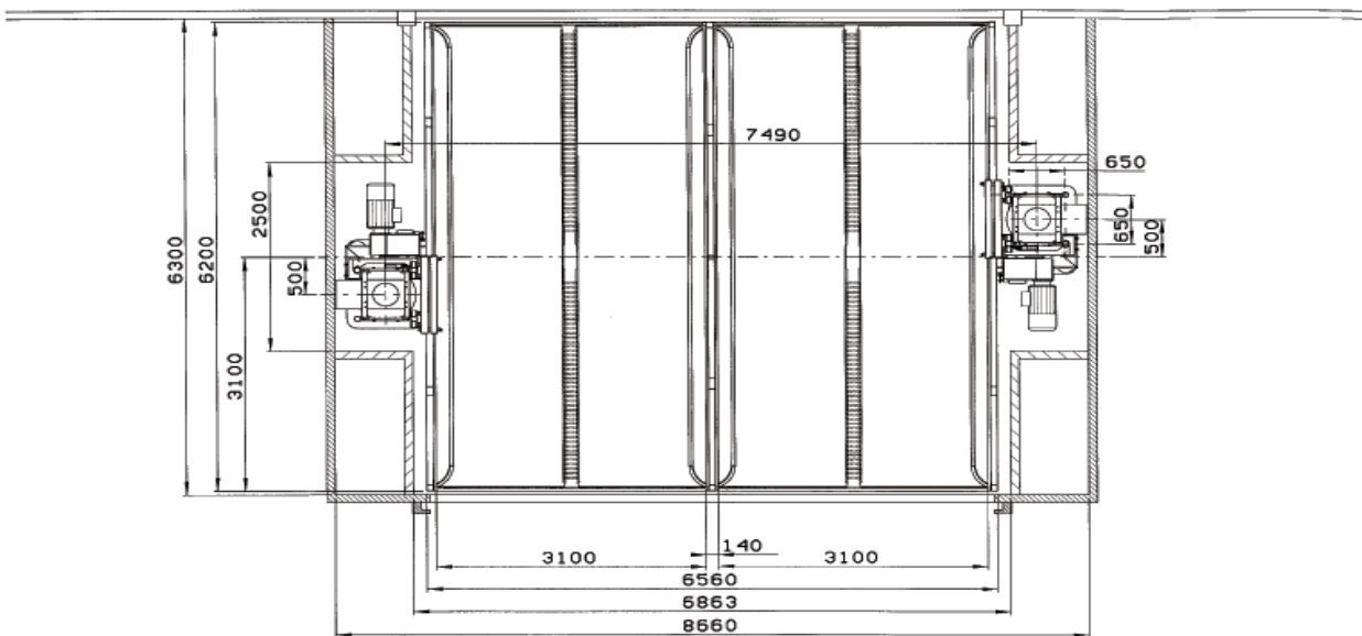
ARK PARKING LIFT TWO MAST VERSION TOP VIEW
